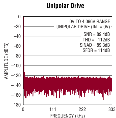
Figure 6e. IN^+ = -1\text{dBFS} 2kHz Unipolar Sine, IN^- = 0\text{V} , 32k Point FFT, f_{\text{SAMPL}} = 666\text{ksps} . Circuit Shown in Figure 6a with LT6237 Amplifiers, R_{\text{FILT}} = 24.9\Omega , C_{\text{FILT}} = 1\text{nF}
