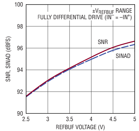
SNR, SINAD vs V_{REFBUF} , f_{IN} = 2\text{kHz}
